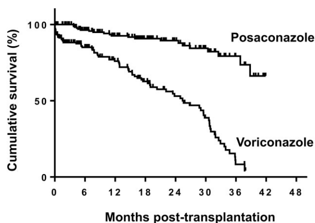
Figure 4. Cox regression analysis of overall survival between the posaconazole group and the voriconazole group.
